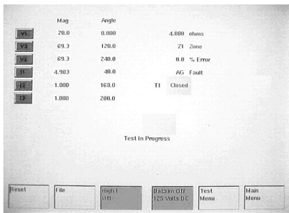
Impedance Reach Test Screen
