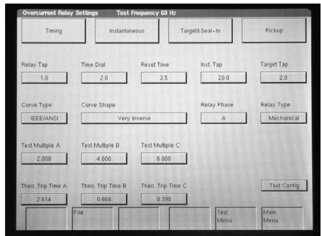
Overcurrent Relay Setting Screen
