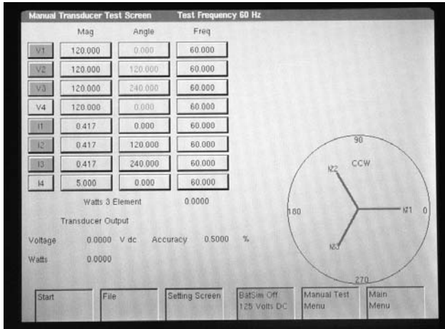
Transducer Test Screen
